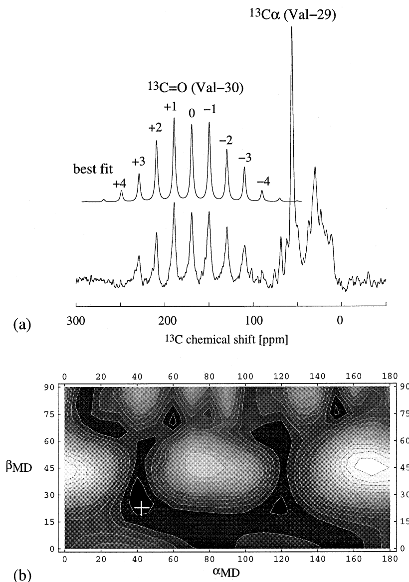
Fig. 6. ^{13}\text{C} -CP-MAOSS NMR spectrum of M13 in DMPC- \text{d}_{67} (L/P=30) at \omega_t=2000 Hz and T=243 K (a). The best-fit search (b) for the spinning sideband pattern of ^{13}\text{C}=\text{O} in Val-29 was carried out in the \alpha_{\text{MD}}/\beta_{\text{MD}} parameter space for different mosaic spread values \Delta\beta , which revealed a average helix tilt of 20^\circ .
