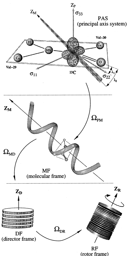
Fig. 5. Reference frames for a carbonyl labelled site in a protein backbone: Two Euler angles are needed to describe the rotations about \sigma_{33} ( \alpha_{PM} = -80^\circ – -90^\circ ) and \sigma_{22} ( \beta_{PM} = 85^\circ – 90^\circ ), which relate the principal axis system of the ^{13}C=O shielding tensor to the peptide plane and so to the molecular reference frame. \lambda_1 and \lambda_2 are the angles between the C=O bond vector and \sigma_{22} and Z_M . The orientation of the helix with respect to the membrane normal is given by the tilt angle \beta_{MD} while an additional rotation about Z_M by \alpha_{MD} fixes the position of the ^{13}C=O label within the helix. The transformation from the director frame into the MAS rotor frame requires averaging over \alpha_{DR} from 0 to 360^\circ to account for the two-dimensional distribution in the membrane, while remaining orientational disorder \Delta\beta is included by \beta_{DR} = \pm \Delta\beta .
